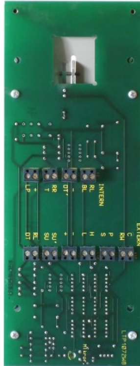
Anschlüsse Platine
